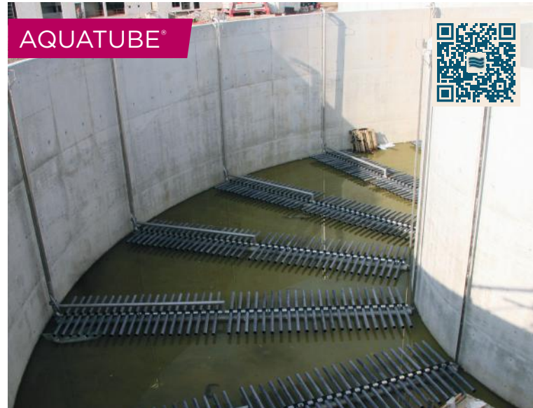
FINE BUBBLE AIR TUBE DIFFUSERS
